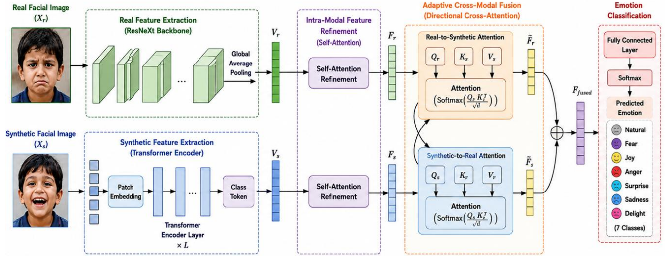
Figure 1. DA-ACFNet Architecture Diagram
