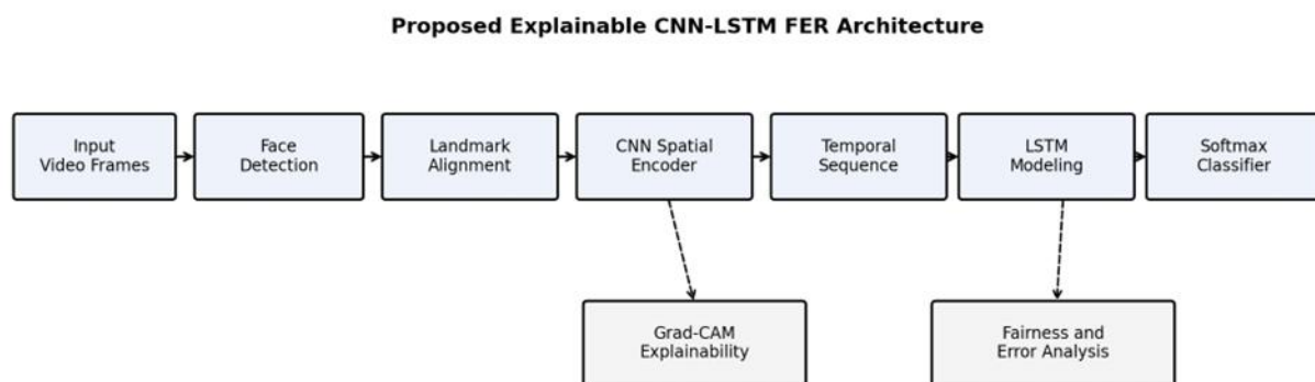
Figure 1. Proposed explainable CNN-LSTM architecture for facial emotion recognition in intellectually disabled children.
