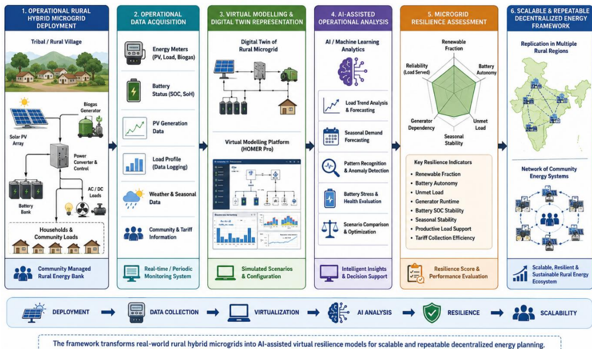
Figure 1. Proposed AI-assisted virtual resilience assessment framework for community-managed rural hybrid microgrids.
